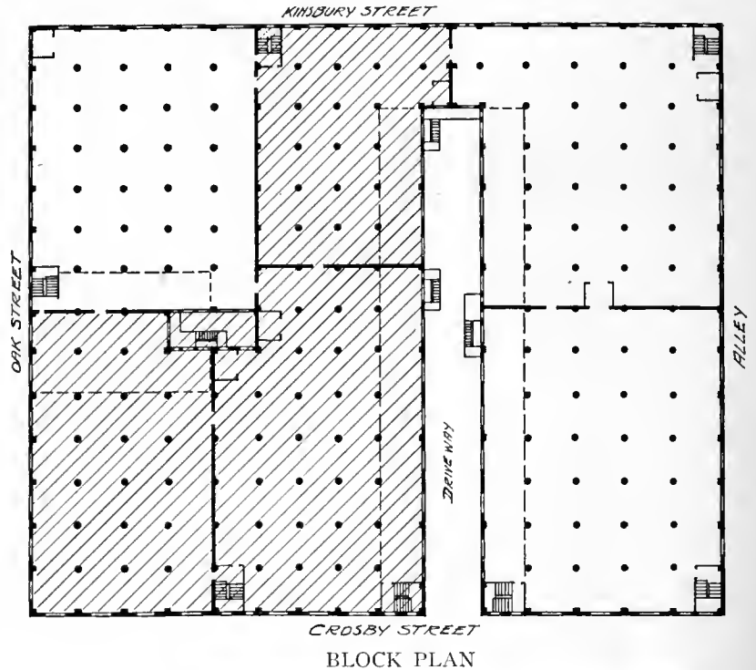
BLOCK PLAN
